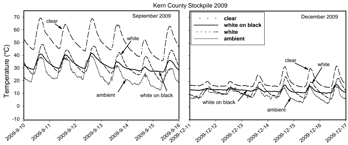
Figure 6. Detailed temperature (in degrees Celsius) near top of stockpile under three different types of plastic cover in Kern County 2009 during mid September (on left) and mid-December (on right). Mid-December included several cloudy days.
