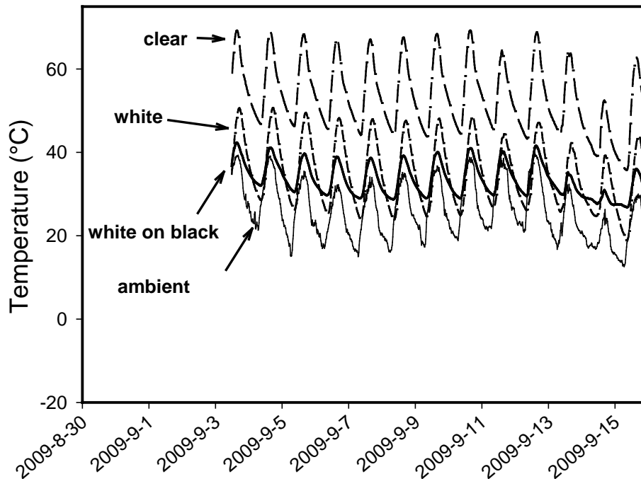
Figure 5. Temperature (in degrees Celsius) near top of stockpile under three different types of plastic cover in Kern County 2009. High temperatures under different tarp materials of 70, 50 and 40 degrees Celsius correspond to 158, 122, and 104 degrees Fahrenheit.
