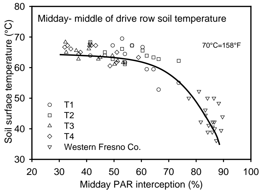
Figure 4. Middle of drive row temperature at midday at varying levels of canopy cover for spur dynamics trial 2003-2004 and hedgerow trial in Western Fresno County.
