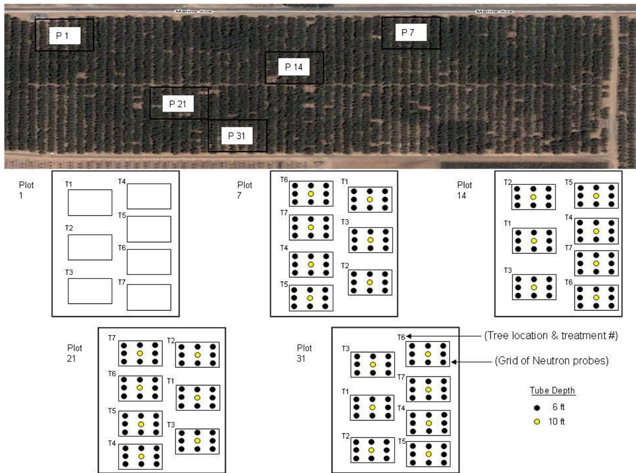
Figure 1. Plot layout at the Nickels Marine avenue site. Each plot contains the 7 drought treatments (see Table 1 ) and one or two control trees (not indicated).
