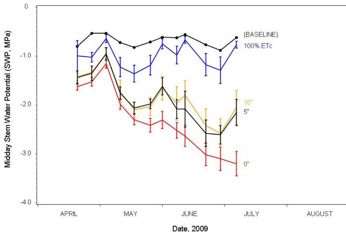
Figure 2. SWP values for the control (100% ETC), and the different drought treatments thus far. Baseline SWP values (those expected for non-stressed almond trees) are also shown.
